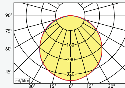
— C0-C180 — C90-C270 Opal
