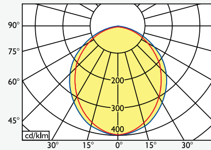
Opal — C0-C180 — C90-C270
